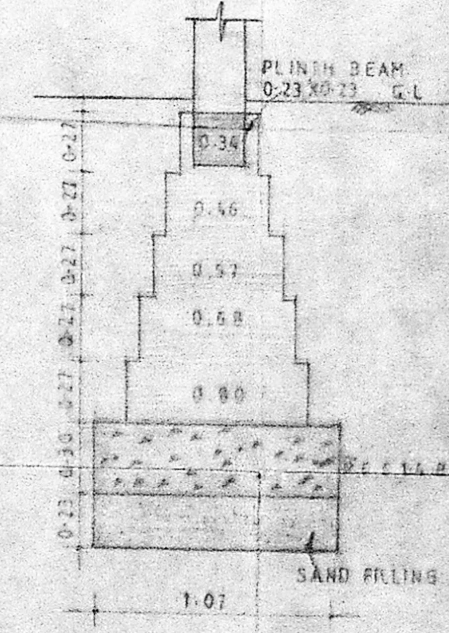
FOUNDATION DETAILS SCALE: 1:25
